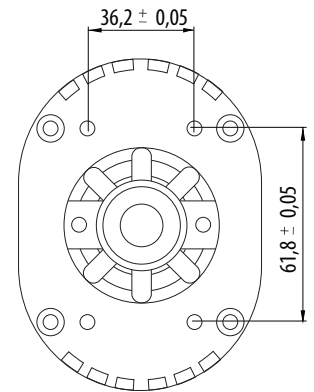
Fixing layout
